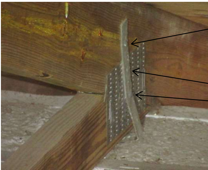
Single strap with at least 3 nails into the truss
